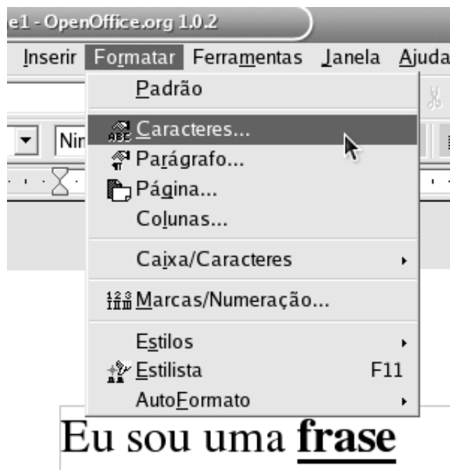
Figura 18.11: Formatar : Caracteres
